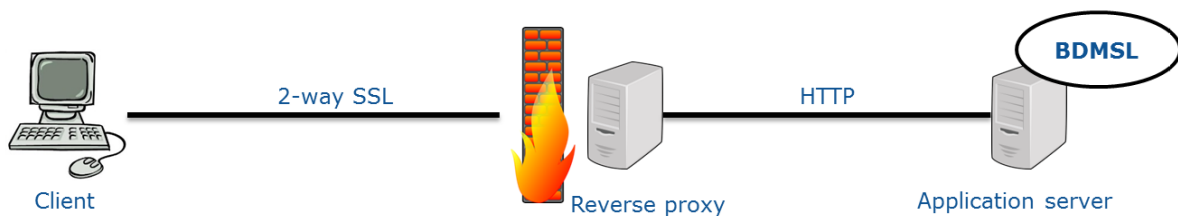
Figure 25 - Reverse proxy with SSL
